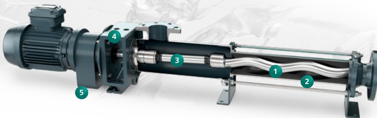
NEMO® industrial
